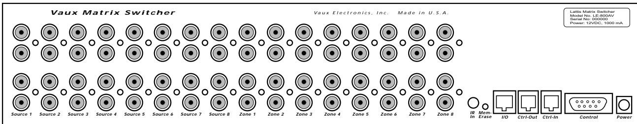
LE-800AV rear panel
